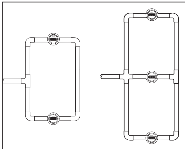
Figure 1. Multiple Body Spray Pressure Balancing Loop
